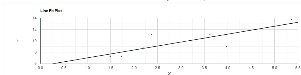
Figure 1. Highest number of rainy days per month correlated with sexual size dimorphism in Sphaerotheriidae Brandt, 1833.
