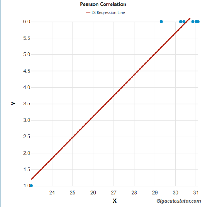
Figure 1. Longitude and species richness correlation in southern African Vaalagonopodidae.
