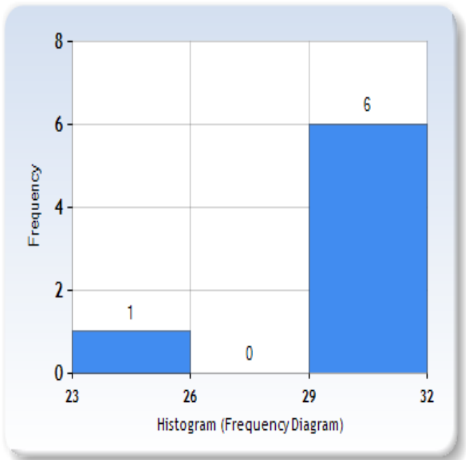
Figure 2. Longitudinal species richness in southern African Vaalagonopodidae.
