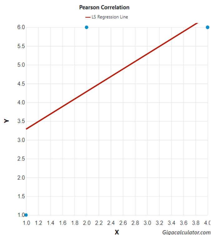
Figure 1. Latitude and species richness correlation in southern African Vaalagonopodidae.
