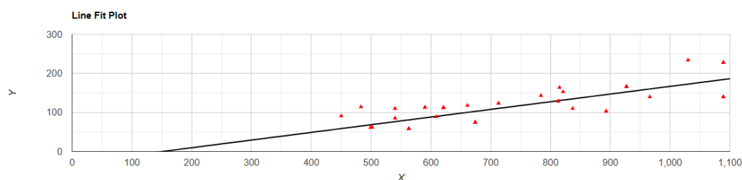
Figure 1. Precipitation correlated with maximum precipitation in Sphaerotheriidae Brandt, 1833.
