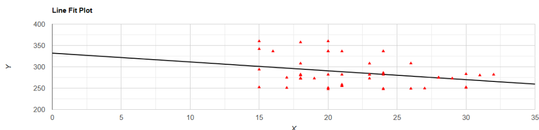
Figure 1. Highest daily hours of sunshine per month correlated with temperature in Sphaerotheriidae Brandt, 1833.
