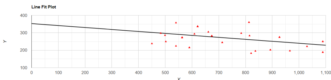
Figure 1. Precipitation correlated with lowest daily hours of sunshine per month in Sphaerotheriidae Brandt, 1833.
