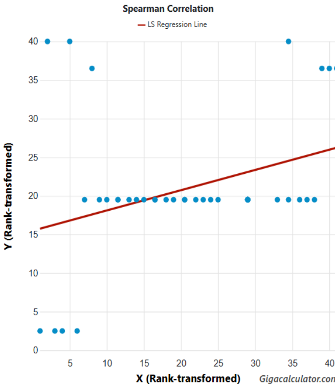
Figure 2. Spearmans correlation between latitude and range in latitude across four genera of the southern African Gomphodesmidae.
