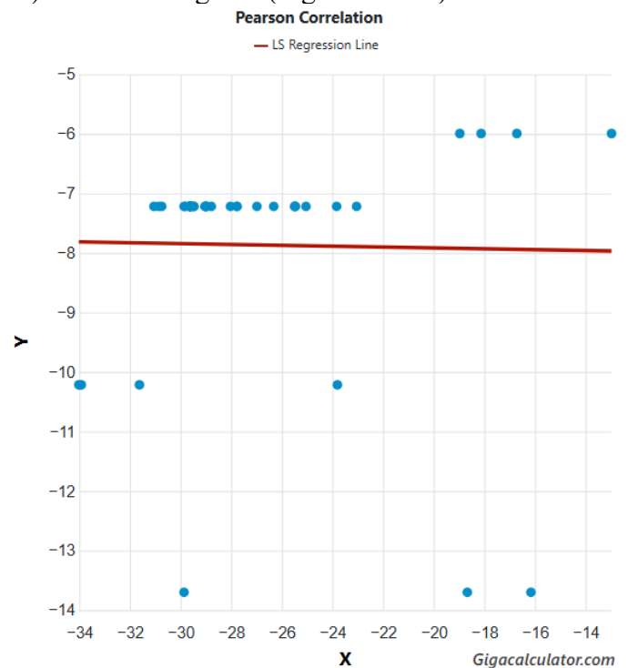
Figure 1. Pearson correlation between latitude and range in latitude across four genera of the southern African Gomphodesmidae.
