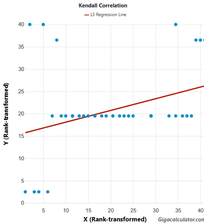
Figure 3. Kendall correlation between latitude and range in latitude across four genera of the southern African Gomphodesmidae.
