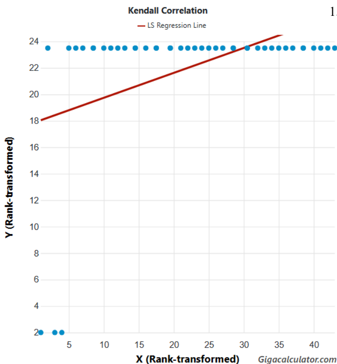
Figure 3. Kendall correlation between latitude and range in latitude across four genera of the southern African Pachybolidae.
