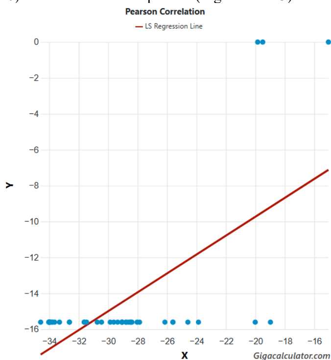
Figure 1. Pearson correlation between latitude and range in latitude across four genera of the southern African Pachybolidae.
