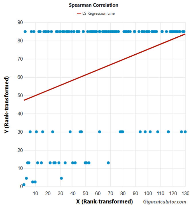
Figure 2. Spearmans correlation between latitude and range in latitude across six genera of the southern African Odontopygidae.
