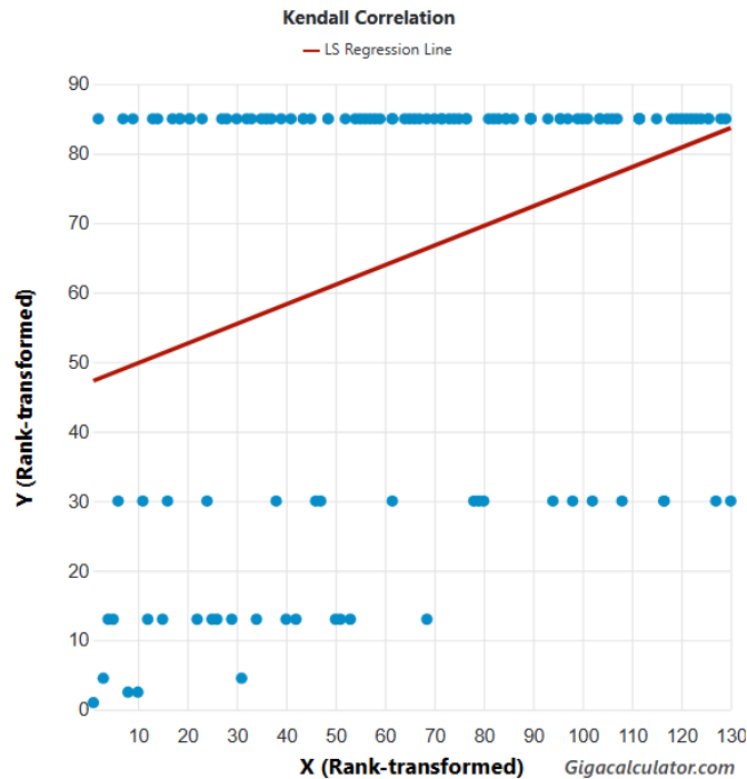
Figure 3. Kendall correlation between latitude and range in latitude across six genera of the southern African Odontopygidae.
