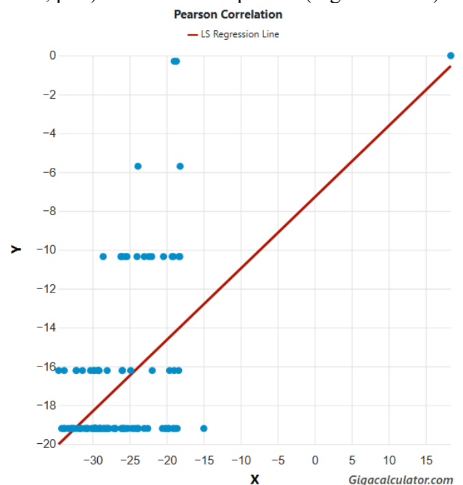
Figure 1. Pearson correlation between latitude and range in latitude across six genera of the southern African Odontopygidae.
