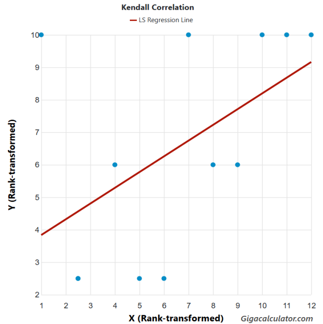
Figure 3. Kendall correlation between latitude and range in latitude across six genera of the southern African Paradoxosomatidae.
