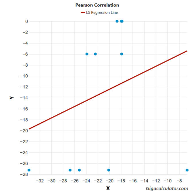
Figure 1. Pearson correlation between latitude and range in latitude across six genera of the southern African Paradoxosomatidae.
