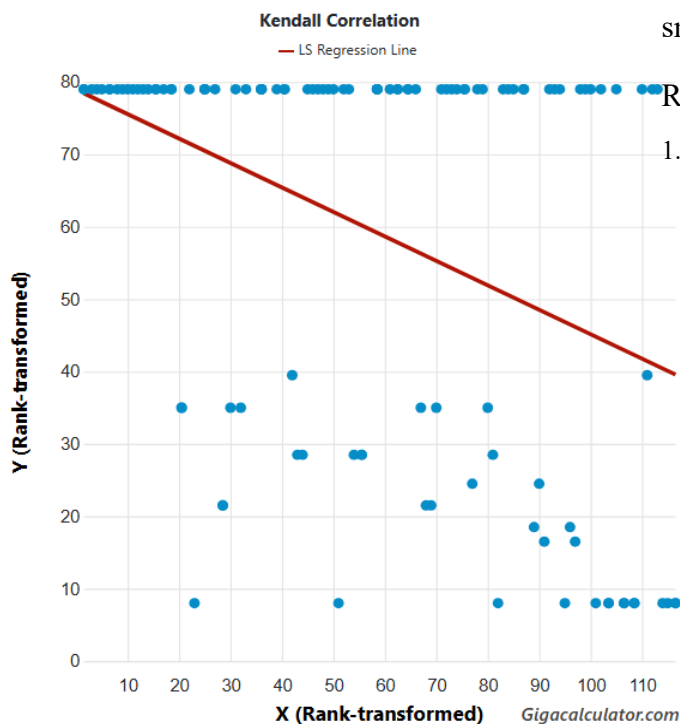
Figure 3. Kendall correlation between latitude and range in latitude across 21 genera of the southern African Dalodesmidae.
