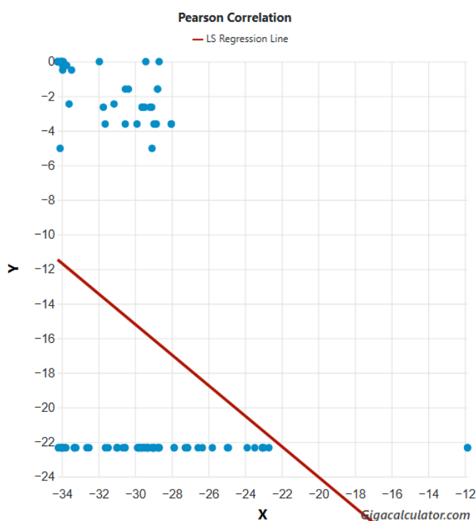
Figure 1. Pearson correlation between latitude and range in latitude across 21 genera of the southern African Dalodesmidae.
