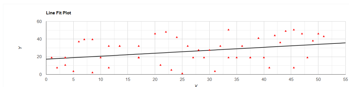
Figure 1. Average temperature variation correlated with altitude in Sphaerotheriidae Brandt, 1833.
