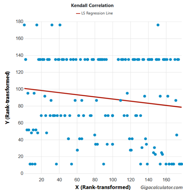
Figure 2. Kendall correlation between latitude and range in latitude across 33 genera of the southern African Polydesmida Leach, 1815.
