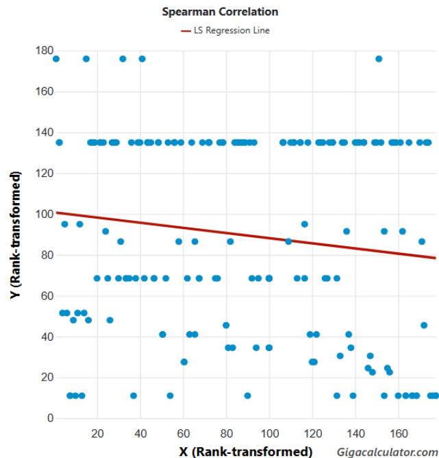
Figure 1. Spearmans correlation between latitude and range in latitude across 33 genera of the southern African Polydesmida Leach, 1815.
