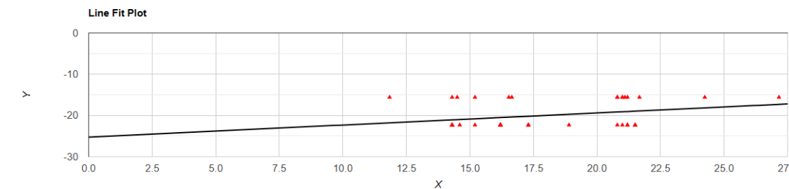
Figure 11. Minimum ocean water temperature correlated with the range in latitude in southern African forest millipedes.
