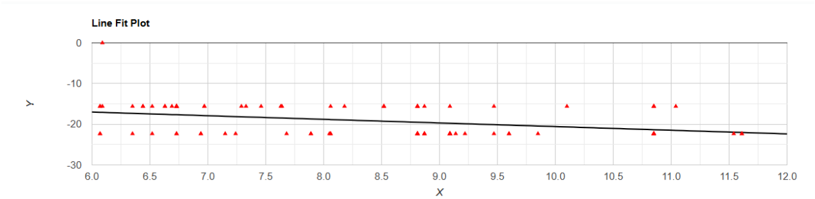
Figure 5. Lowest daily hours of sunshine per day correlated with the range in latitude in southern African forest millipedes.
