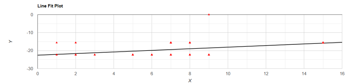
Figure 10. Longitudinal species richness correlated with range in latitude in southern African forest millipedes.
