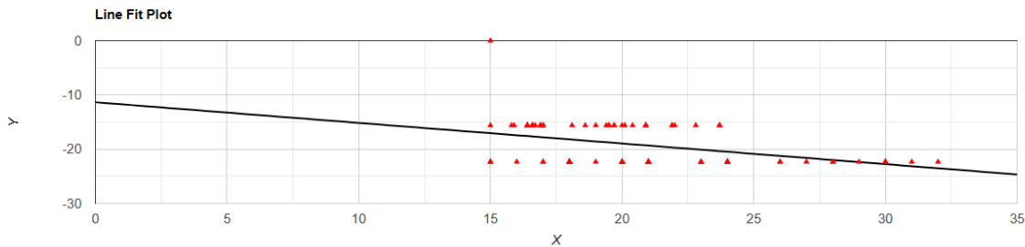
Figure 1. Temperature correlated with range in latitude in southern African forest millipedes.
