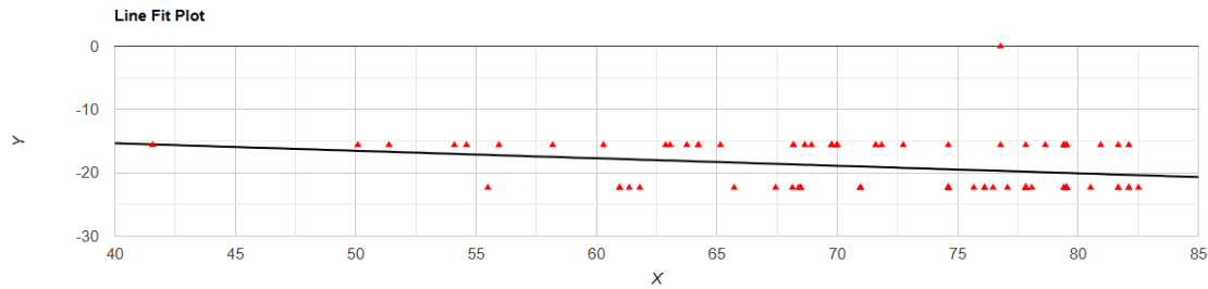
Figure 4. The highest relative humidity correlated with the range in latitude in southern African forest millipedes.
