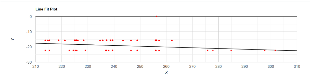
Figure 8. Average monthly duration of sunshine correlated with the range in latitude in southern African forest millipedes.
