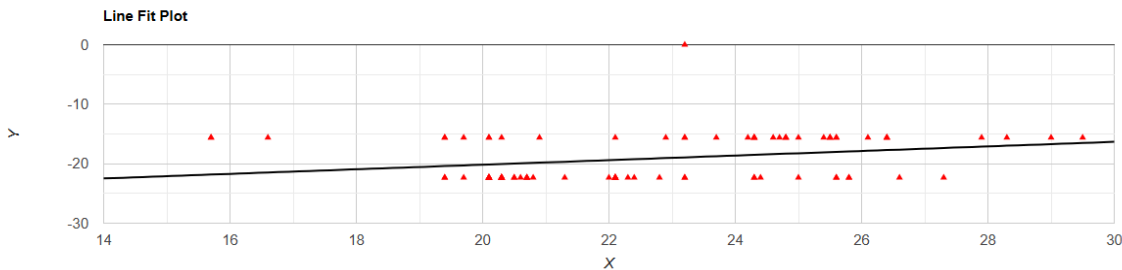
Figure 2. Maximum temperature correlated with range in latitude in southern African forest millipedes.
