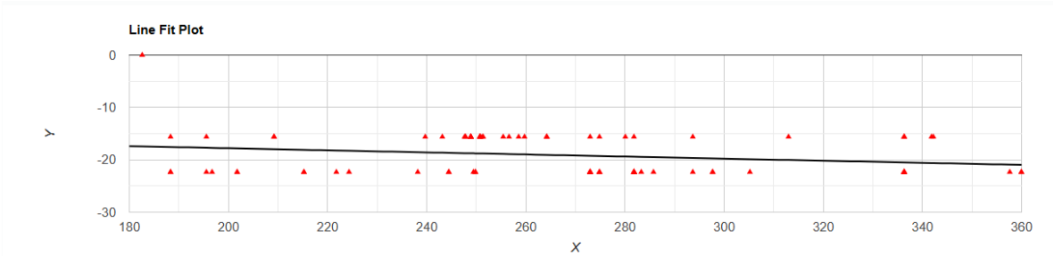
Figure 6. Lowest daily hours of sunshine per month correlated with the range in latitude in southern African forest millipedes.
