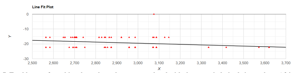
Figure 7. Total hours of sunshine throughout the year correlated with the range in latitude in southern African forest millipedes.
