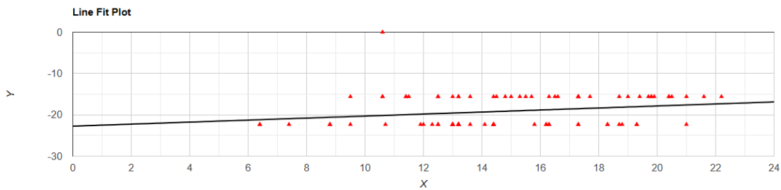
Figure 3. Minimum temperature correlated with range in latitude in southern African forest millipedes.
