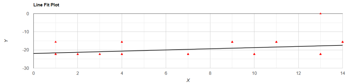
Figure 9. Latitudinal species richness correlated with range in latitude in southern African forest millipedes.
