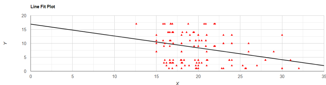
Figure 1. Temperature correlated with latitudinal species richness in South African millipedes.
