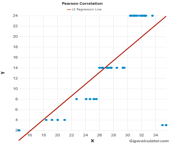
Figure 1. Longitude versus species richness in southern African Spirostreptidae Pocock, 1894.
