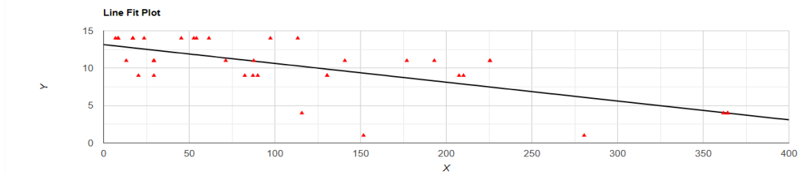
Fig. 1. Correlation between distance to the nearest airport (x) and latitudinal species richness (y) across the range of Centrobolus Cook, 1897.
