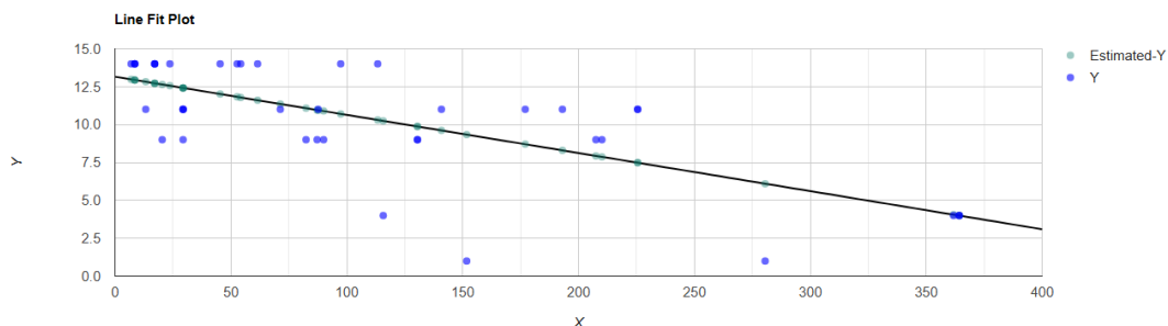
Fig. 2. Regression between distance to the nearest airport (x) and latitudinal species richness (y) across the range of Centrobolus Cook, 1897.
