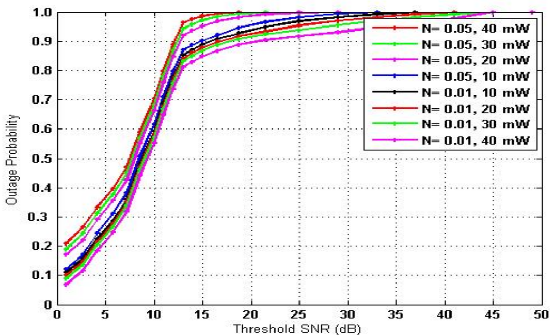
(a) Outage Probability for different noise levels at various value of transmitted power
