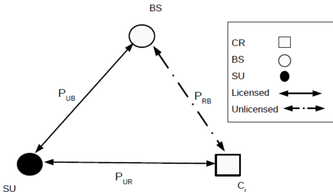
Figure 1. Hybrid Cooperative Relay Network [22]
