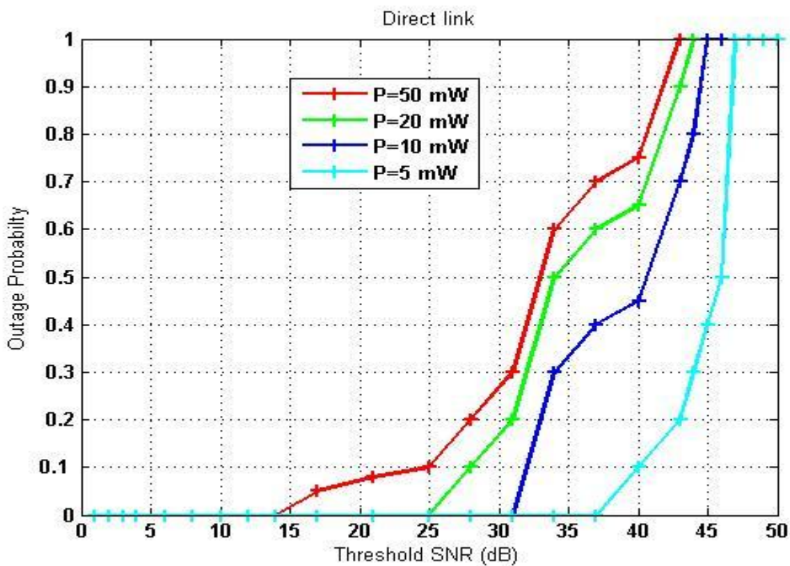
Figure 4: Outage probability versus threshold SNR for several values of transmit power
