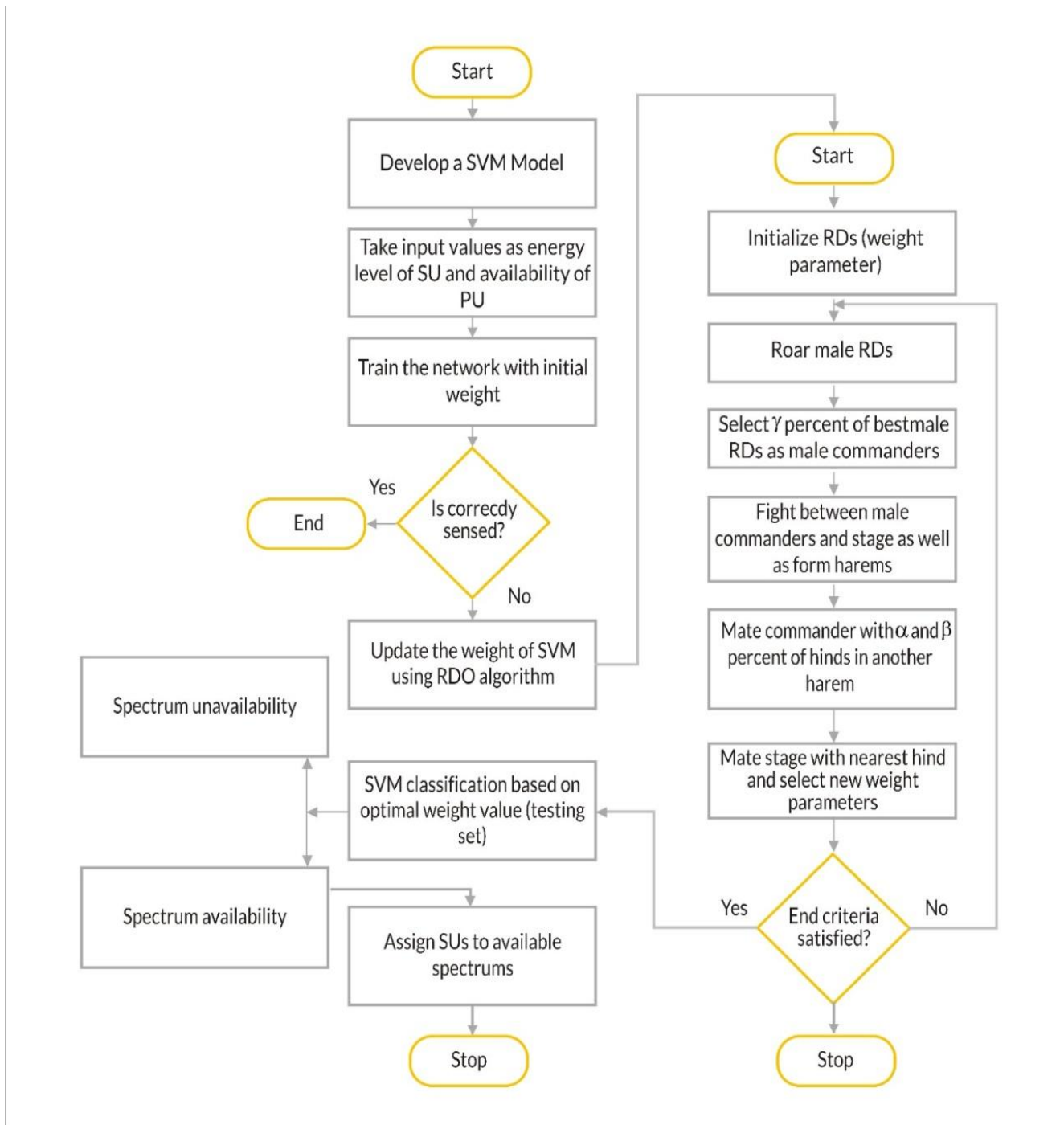
Figure 2 SVM-RDA [22]
