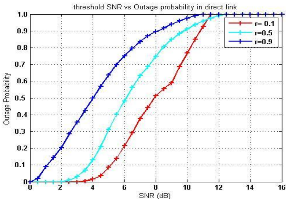
(b) Threshold SNR vs outage probability in direct link
