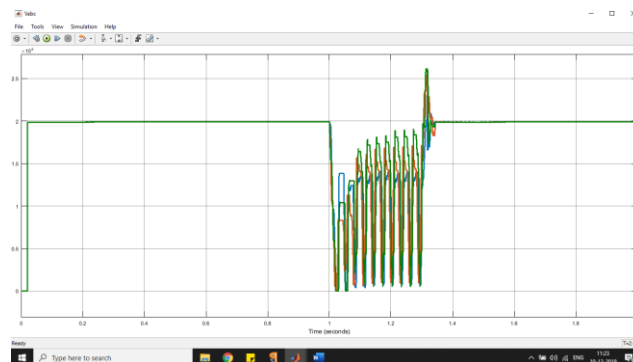
Fig. 4 PVA voltages with over current relay protection with fault from 1 to 1.3sec
