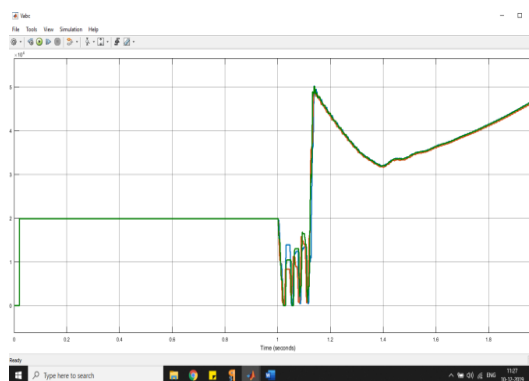
Fig. 6 PVA voltages with over current relay protection with fault from 1 to 1.3sec
