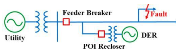
Fig. 2 Proposed system of Fault Characteristic of DER System
